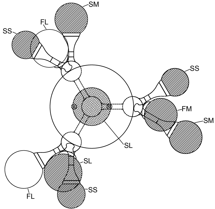
TOP VIEW
